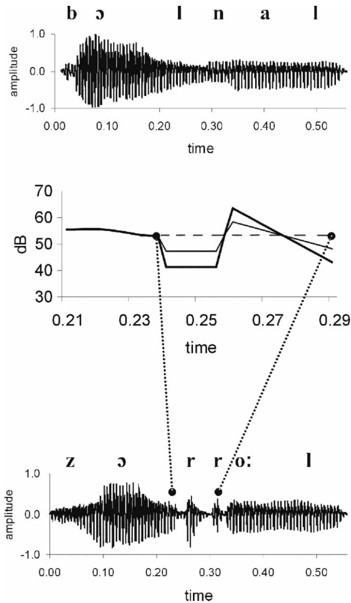
Figure 1. The top panel shows the stimulus “balnal” without AM. The short silence at the beginning is due to the shortening of the prevoice bar. The middle panel shows the parameters used to create AM during the /l/ in “bal” and “zal”. The bottom panel shows the result of this editing, but here with the nonword stimulus “zarrol”. The first AM at 0.265 s is due to the manipulation of an original lateral, while the second peak at 0.315 s stems from the natural suffix “rol”.
